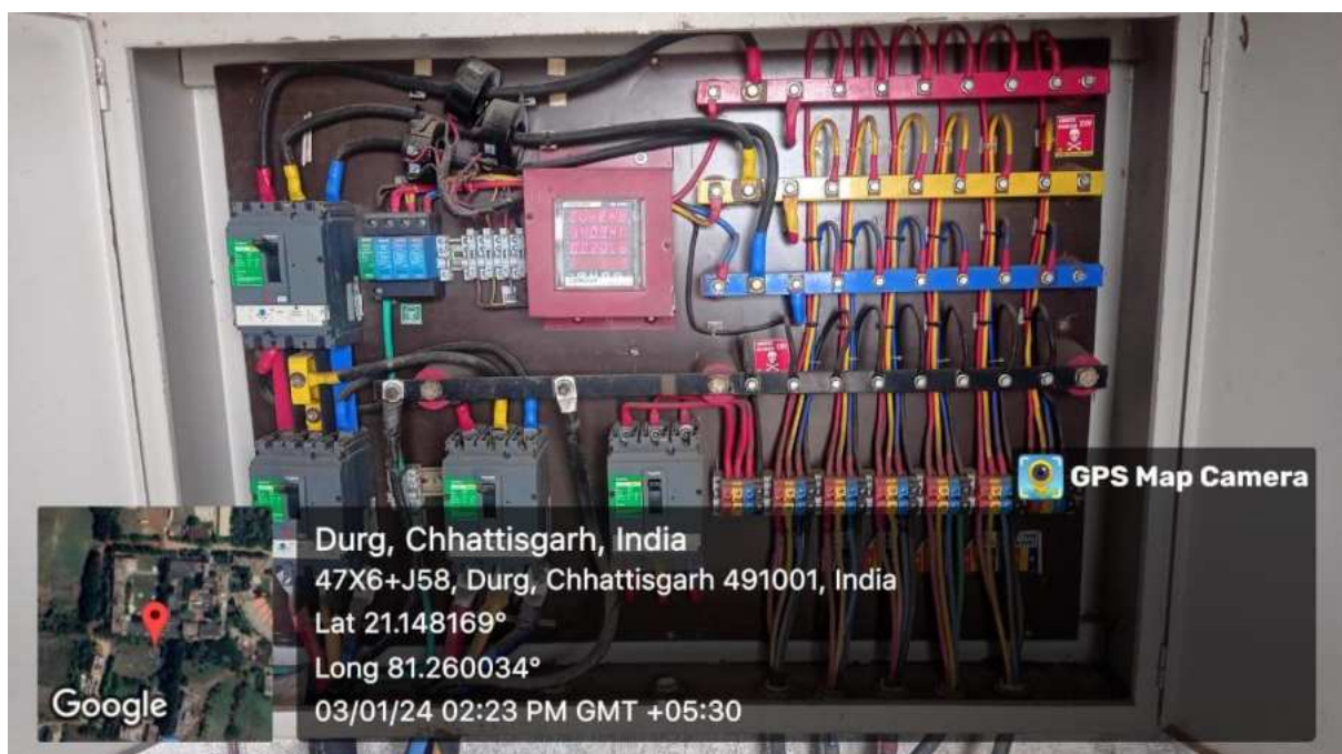
Main Circuit Panel of Solar with readings
